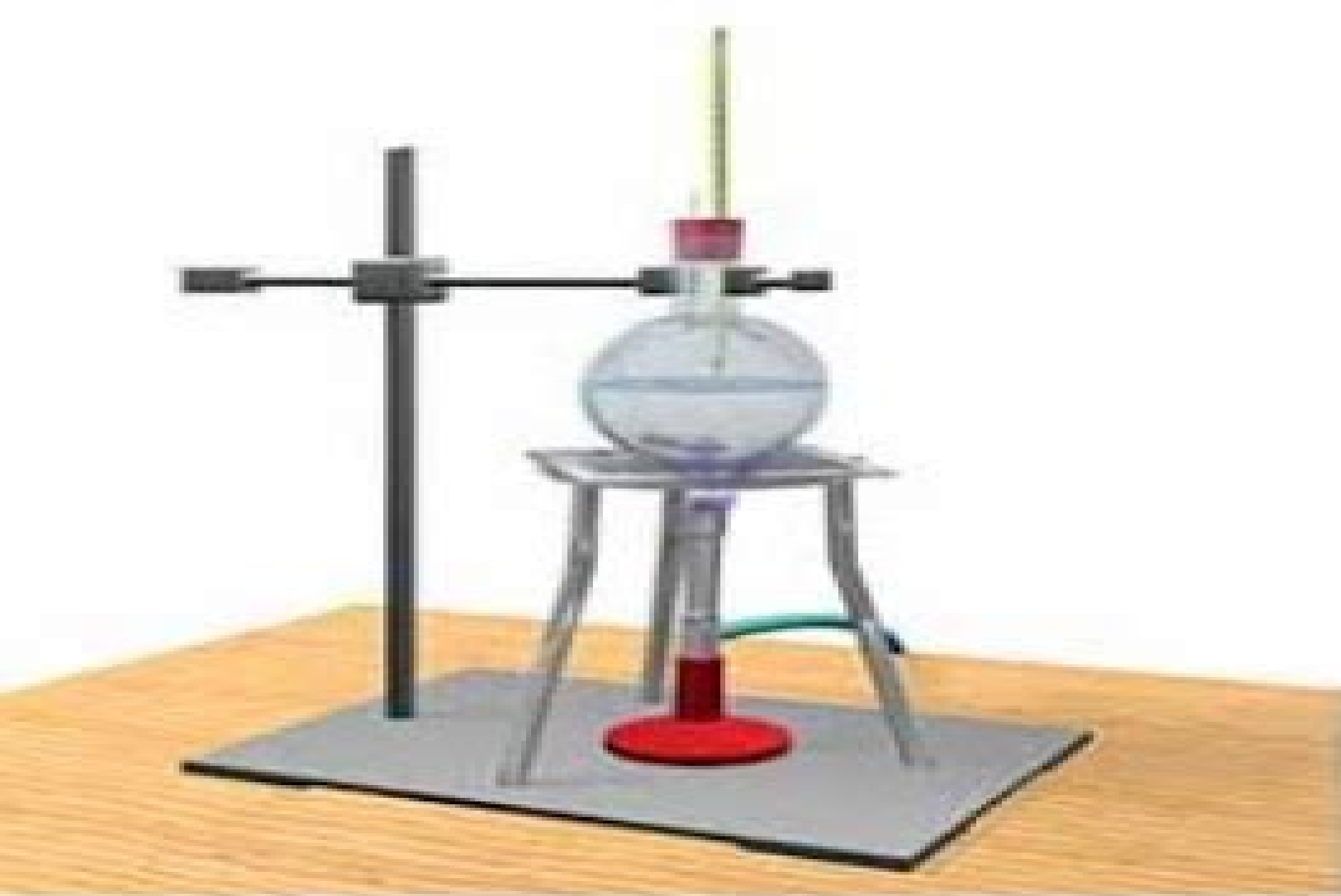
Fig 1: Determination of Boiling point of water
