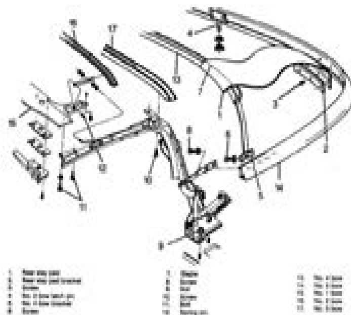
Fig. 7: Convertible top installation
