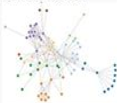
Force-Directed Graph
