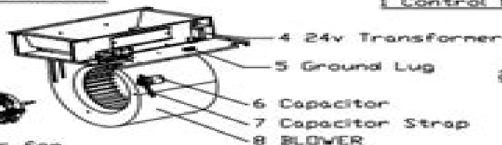
Fig. 22 – FFMA and FMA4 (Sizes 30 &amp; 36) Expanded View - Duct Components, Blower &amp; Electrical Parts
