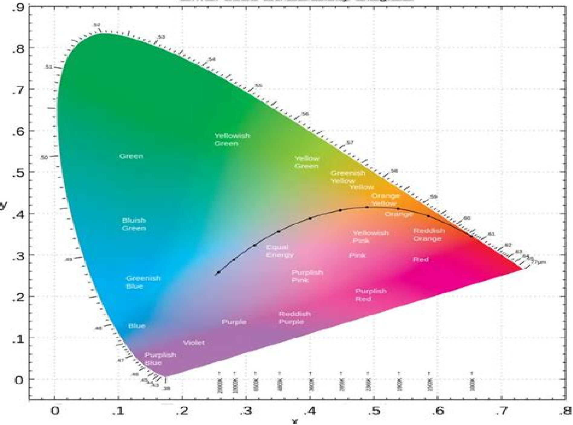
C.I.E. 1931 Chromaticity Diagram
