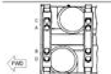
Illustration 21 gm70000 See tightening sequence for the main bearing cap.
