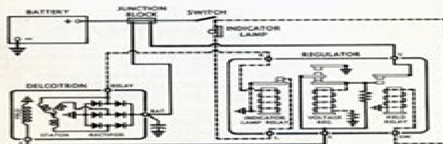
Figure 2—Typical wiring diagram showing internal circuits.
