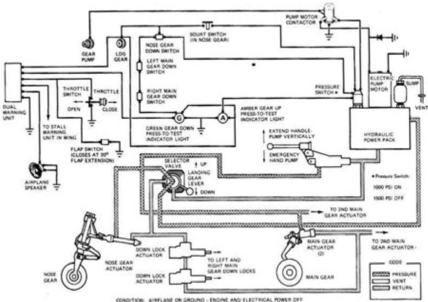
Figure 7-7. Hydraulic System
