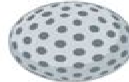
Silica nanoparticle
