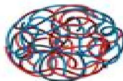
Nanosphere
