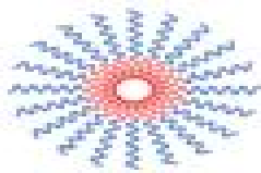
Polymeric micelle
