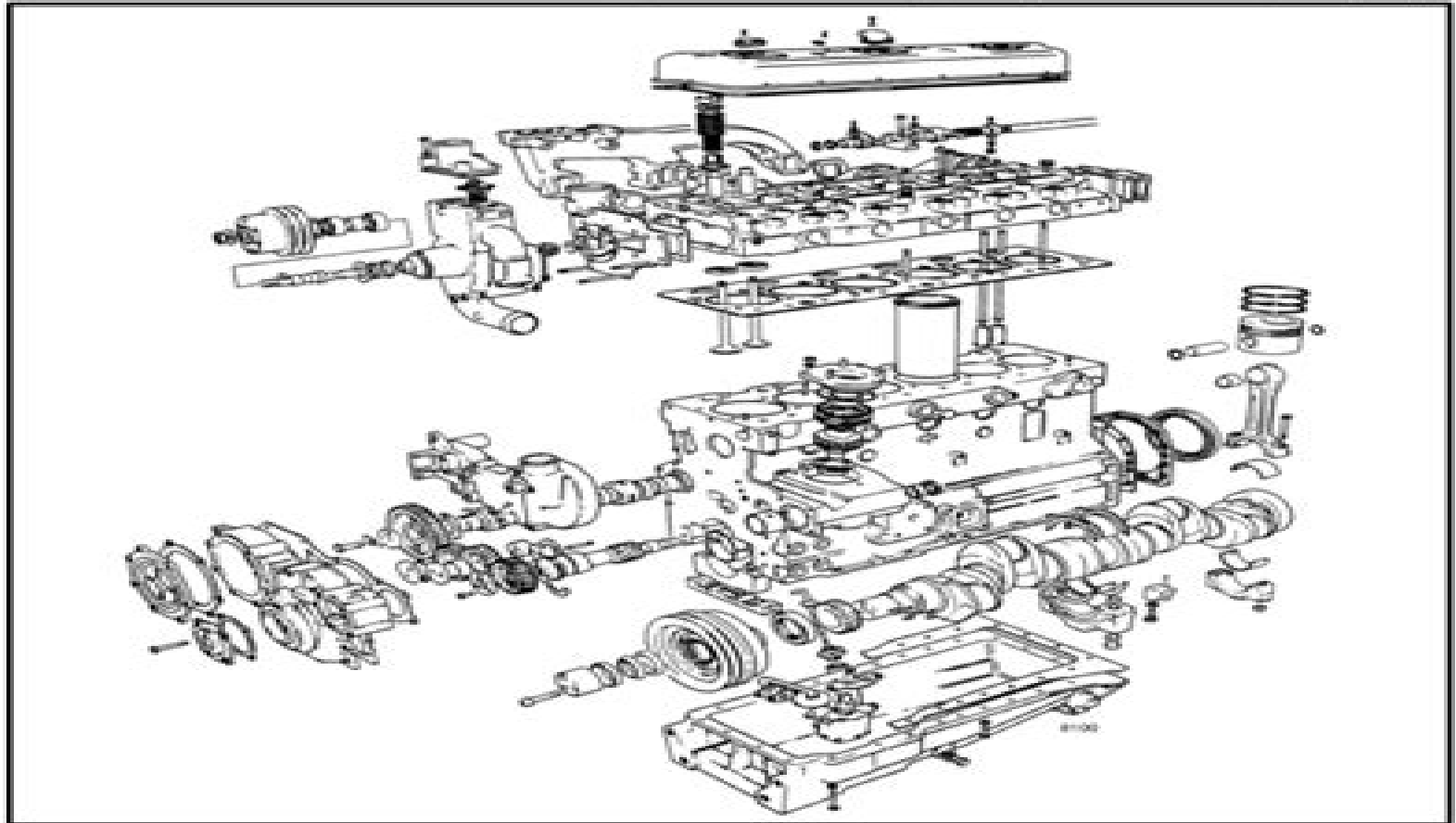
FIGURE 1. PERKINS 6.3544 ENGINE
