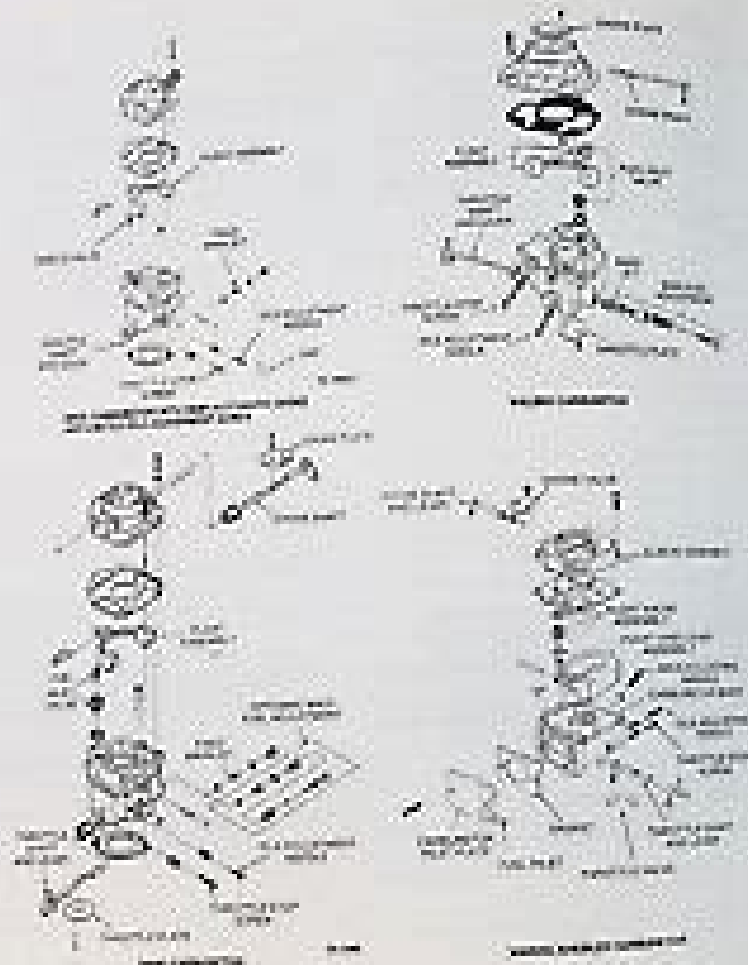
FIGURE 4. CARBURETOR ASSEMBLY
