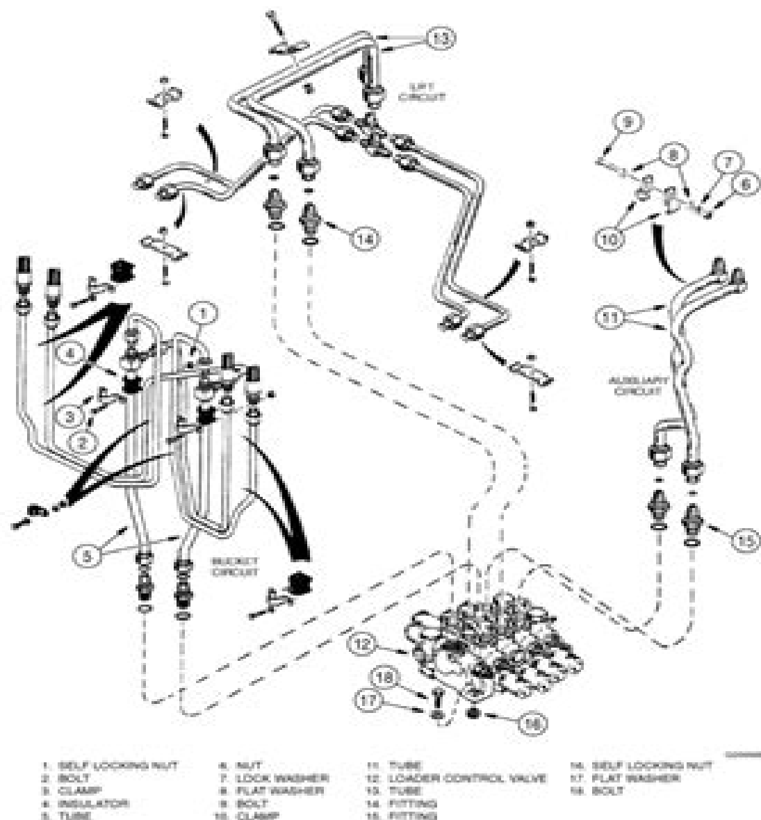
FIGURE 7. XT LOADER CONTROL VALVE REMOVAL AND INSTALLATION
