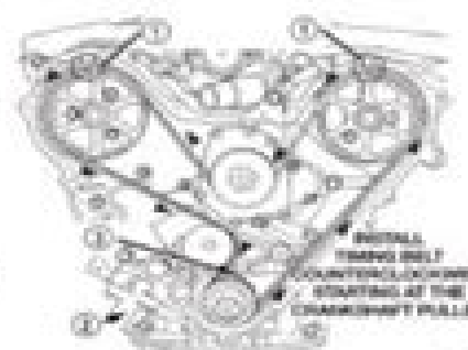
Fig. 76 Timing Belt—Installation
