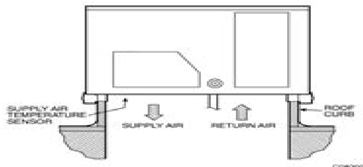
Fig. 42 - Typical Mounting Location for Supply Air Temperature (SAT) Sensor on Small Rooftop Units
