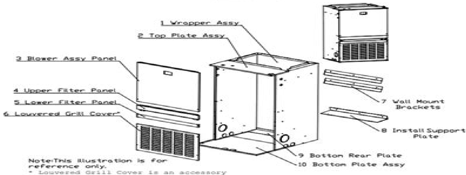
Fig. 21 - FFMA and FMA4 (Sizes 30 &amp; 36) Expanded View - Case
