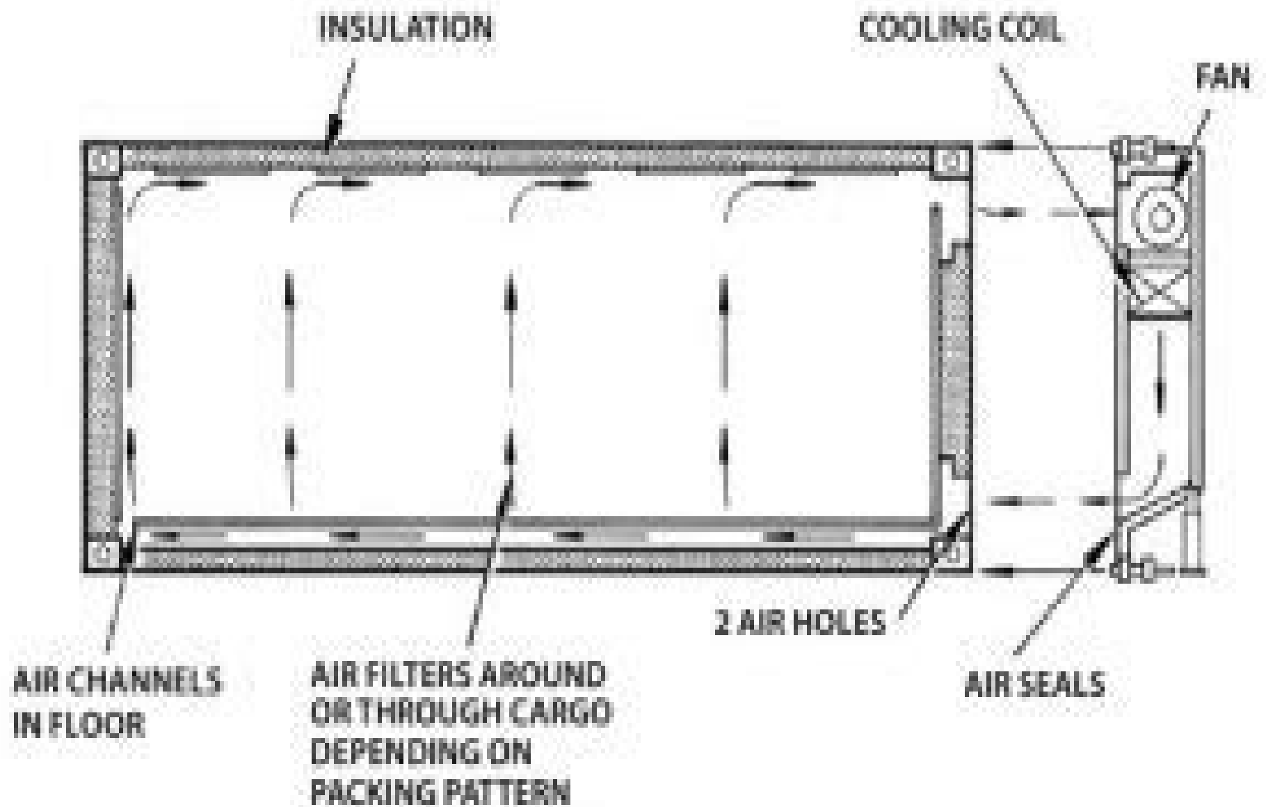
Insulated container requiring external refrigeration source. Bottom air delivery.
