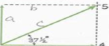
Figure 3.4 \Delta The 3-unit and 4-unit vectors add to produce a resultant vector of 5 units, at 37.5^\circ from the horizontal.
