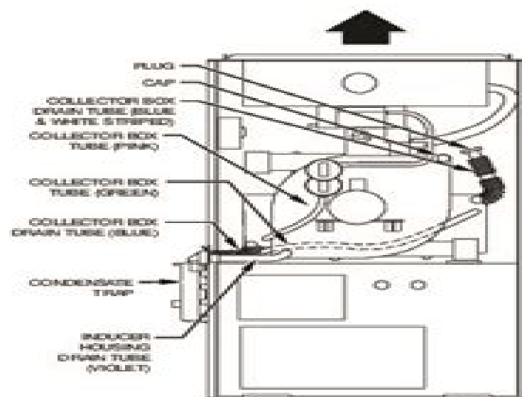
Fig. 7 - Alternate Upflow Configuration and Trap Location
