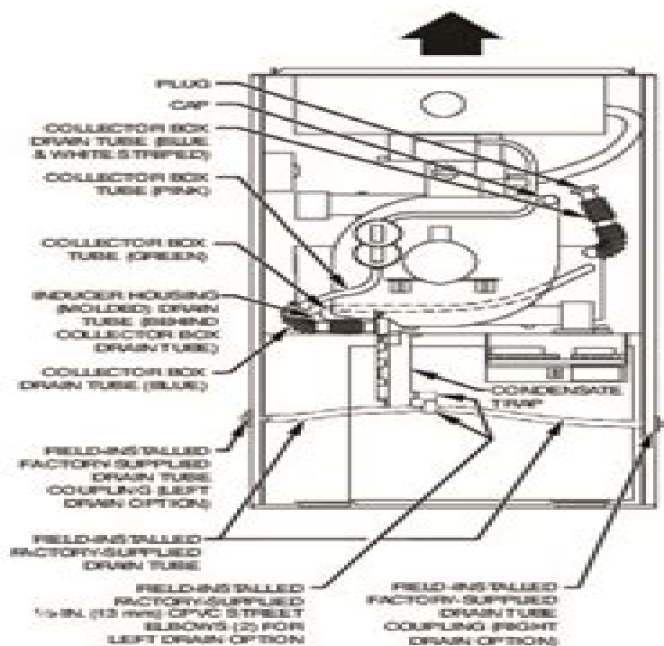
Fig. 6 - Factory-Shipped Upflow Tube Configuration (Shown with Blower Access Panel Removed)
