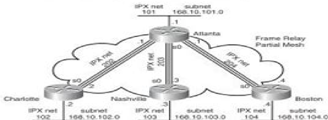
Figure 8-42 Scenario 8-2 Network Derived from show and debug Commands
