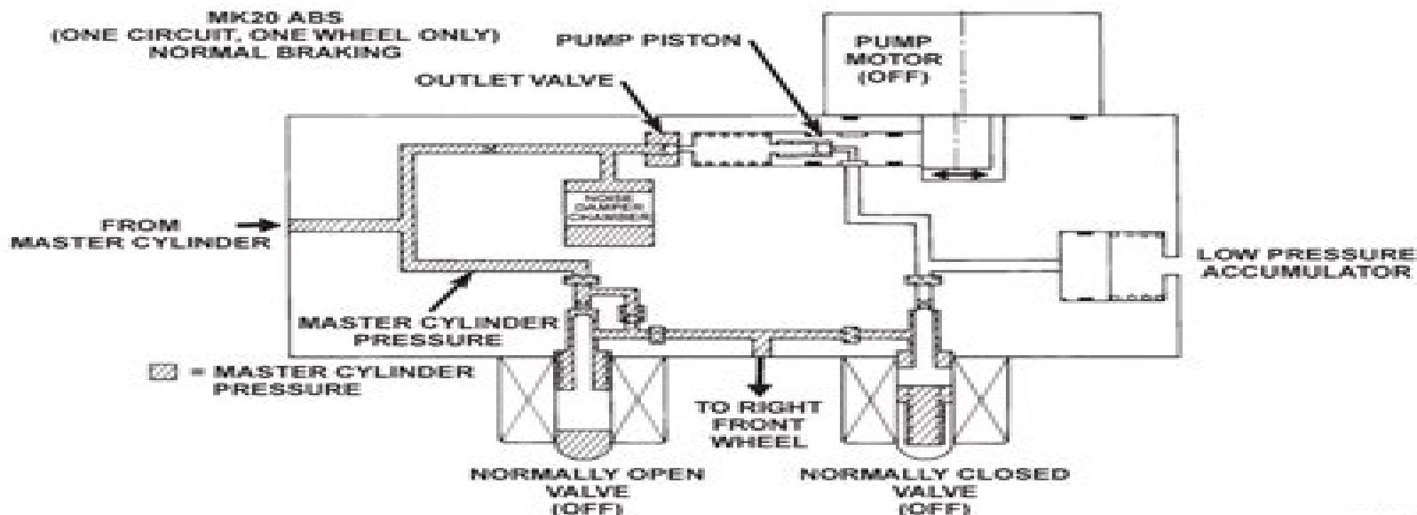
Fig. 11 Normal Braking Hydraulic Circuit
