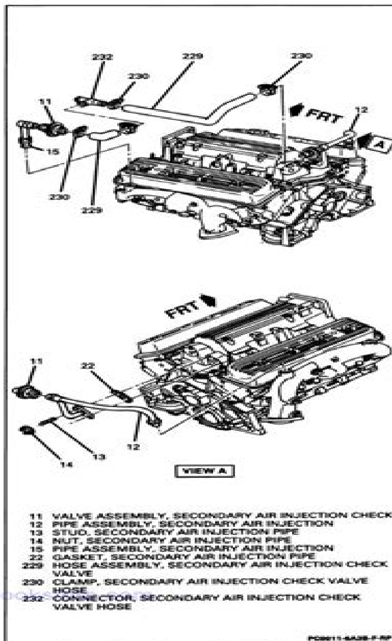
Figure 7 - Secondary Air Injection Components
