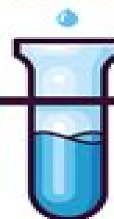
HEMOCYANIN
