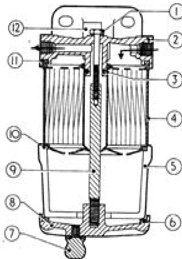
Fig. 12. Agglomerator, Type F.A.S. in section.
