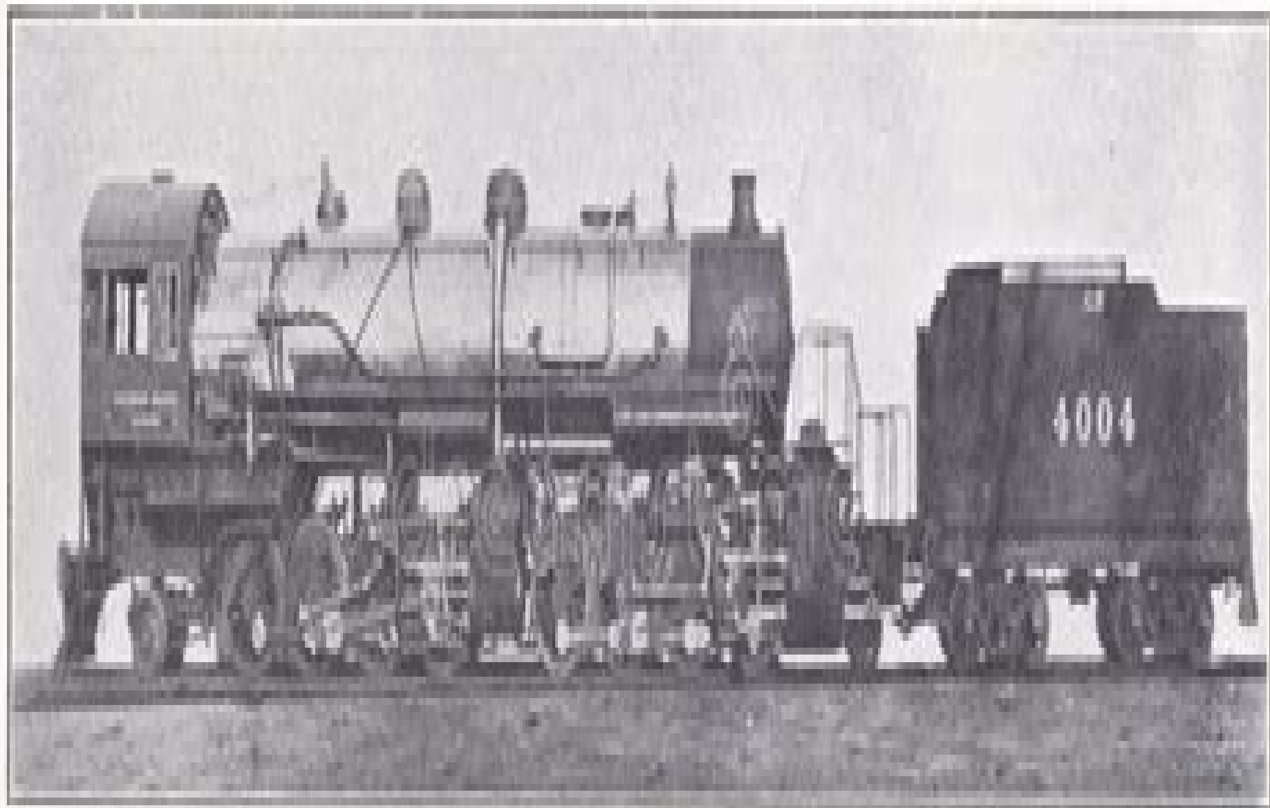
4004 Mallet articulated compound locomotive, Southern Pacific Ry. (see preceding page).
