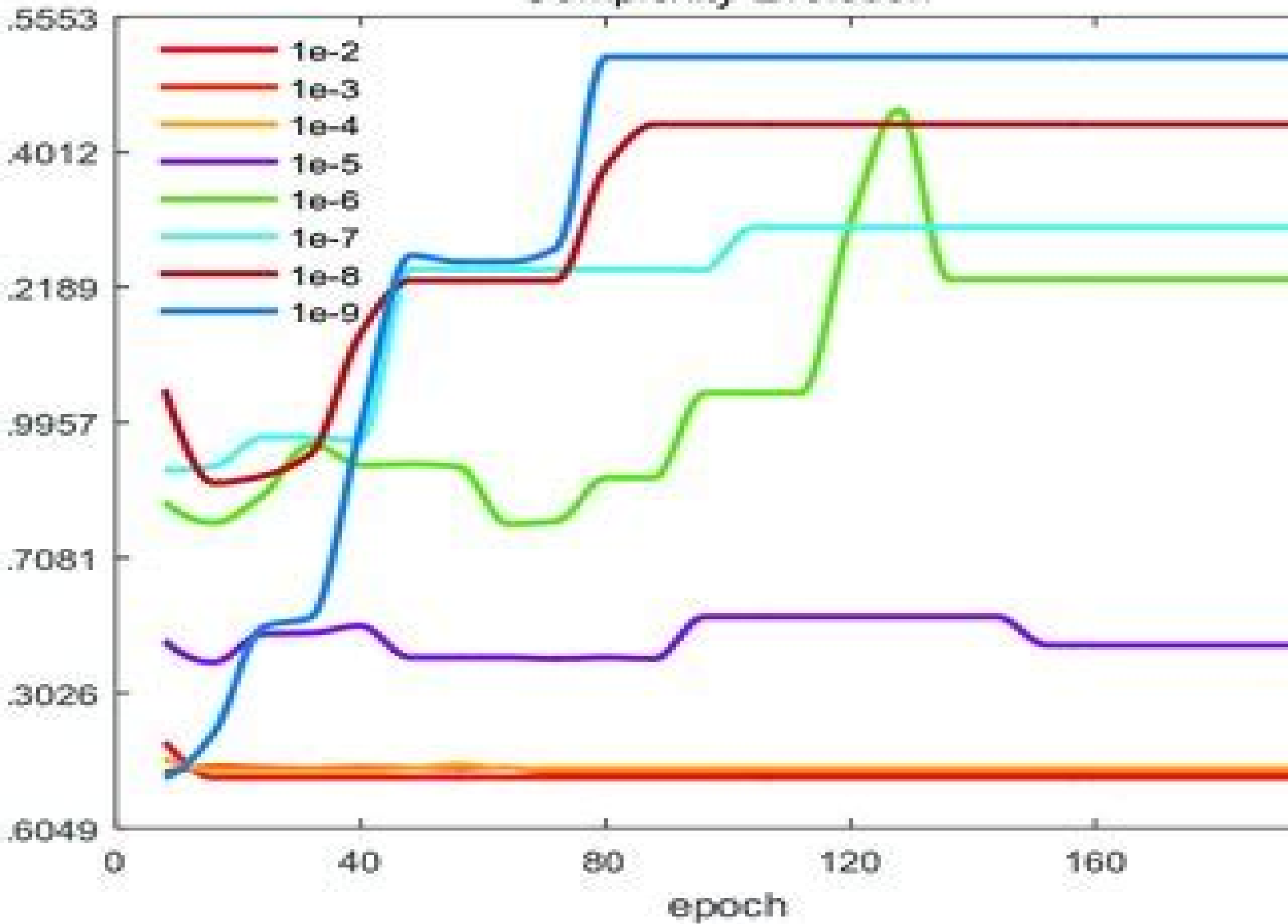
Complexity Evolution
