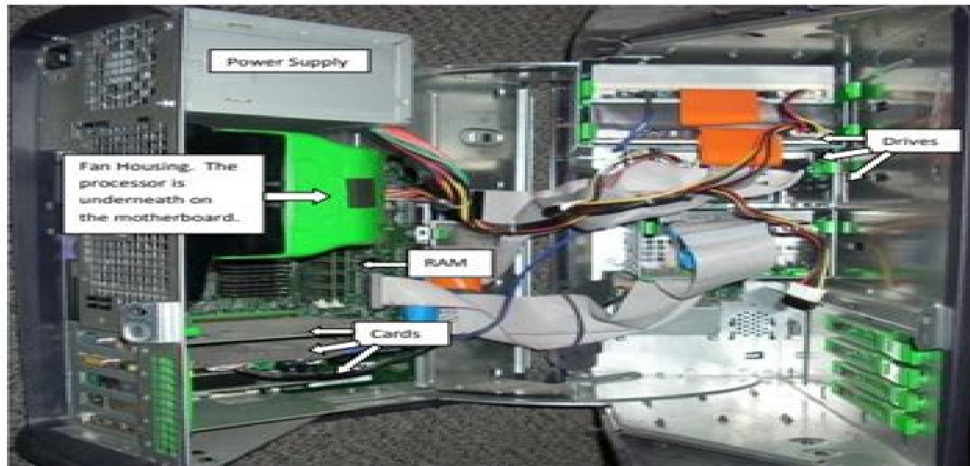
Figure 1 - Inside a Desktop Computer Case
