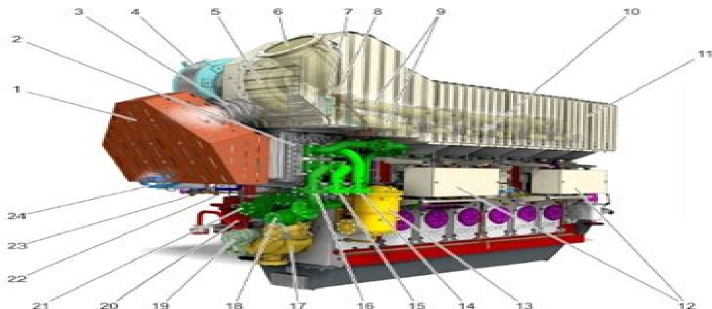
Fig. 2-6 Engine M 25 C, overview of the free end, exhaust side, units and connection points
