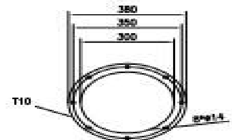
silo bottom outlet drawing 1:120
